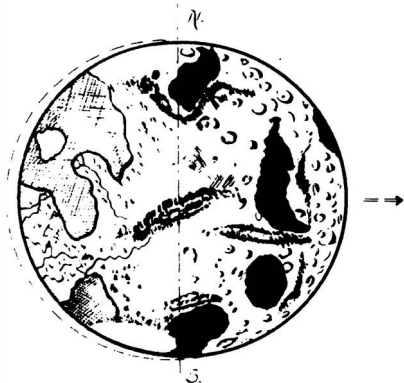
Fig. 9. The astronomer Hansen believed the moon egg-shaped, not spherical, the tip pointing toward Earth. The far side, being "lower," had collected atmosphere. Arrow points toward Earth. Newcomb showed the moon is almost spherical.
