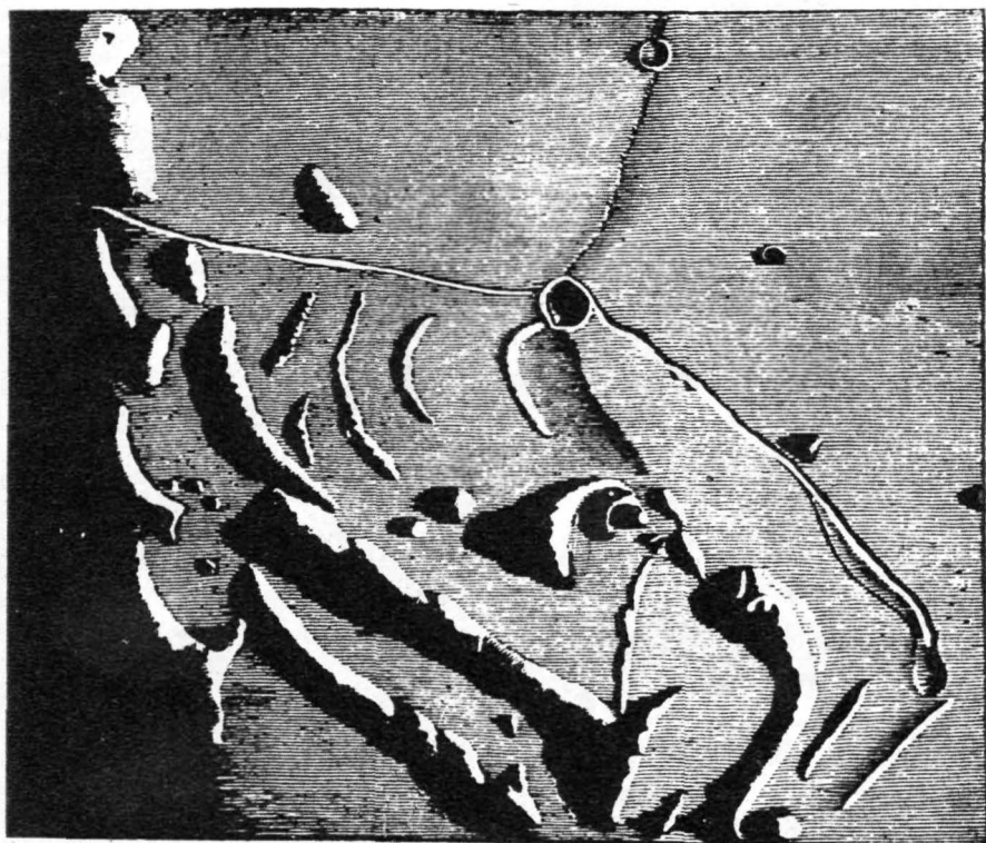
Fig. 10. Section of Moon near Hyginus Chasm, seen near sunset. It creates the impression of some other formation, drowned in hardened lava. The drowned formation is, however, of a type unknown anywhere on Earth.
