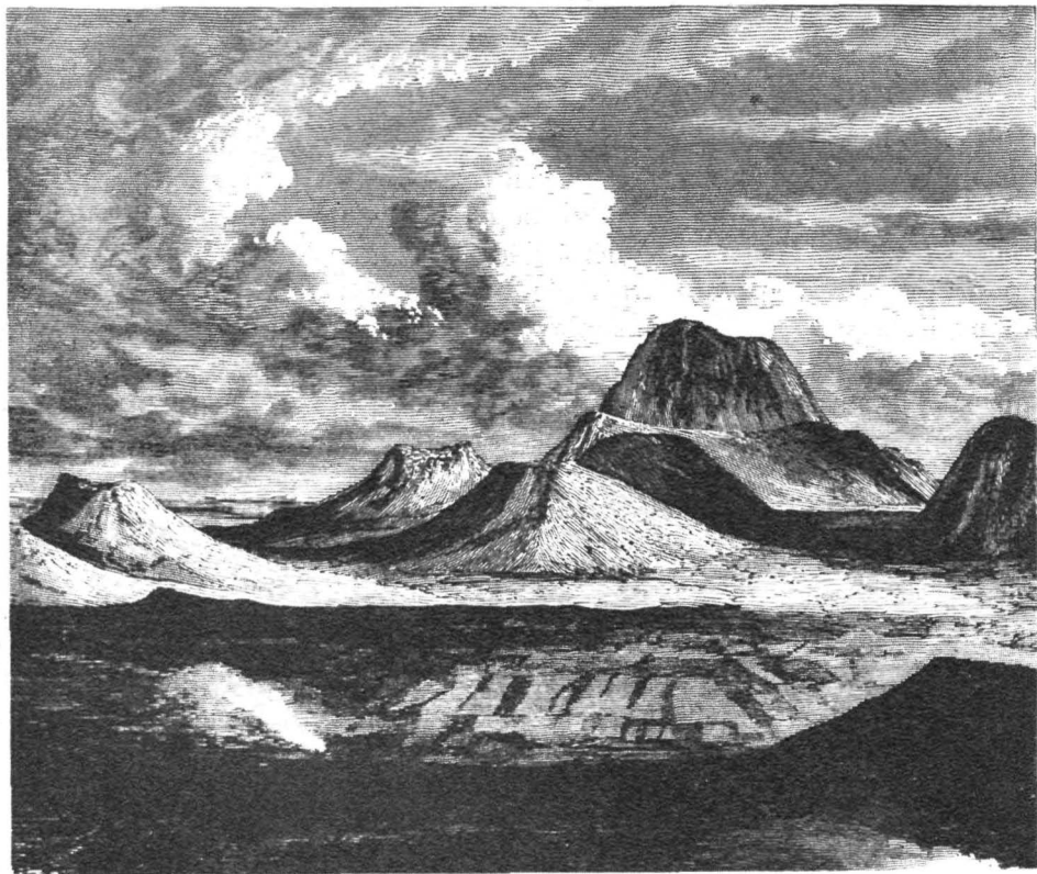
Fig. 3. The model for Flammarion's Lunar landscape, shown in Astronomie Populaire , were these extinct volcanoes in the Auvergne, in France.
