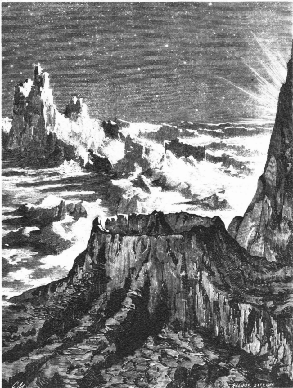
Fig. 2. The astronomer Flammarion pictured the Lunar landscape as a twisted, volcanic area; the true nature of the craters was not known.
