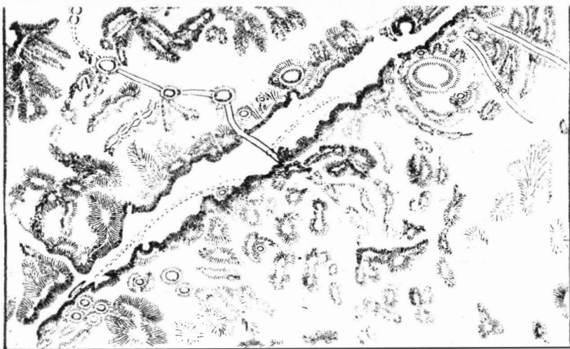
Fig. 7. The "Great Valley" of the Lunar Alps, drawn by Ph. Fauth.
