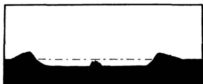
Fig. 6. Top: Cross section of experimental impact crater, the dotted line showing ground level before impact, white line in crater the distribution of the "meteorite." Bottom: Cross section of actual moon crater with central mountain; line as above.
